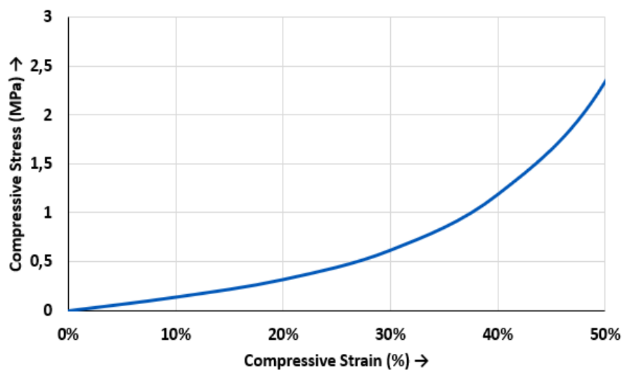
CCL Olympic 7400TW – Compressive Stress vs. Strain
