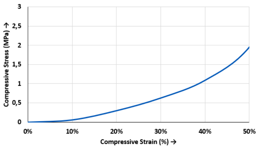
CCL Olympic 8400TW – Compressive Stress vs. Strain
