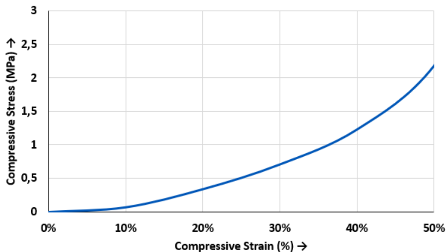
CCL Olympic 8500TW – Compressive Stress vs. Strain
